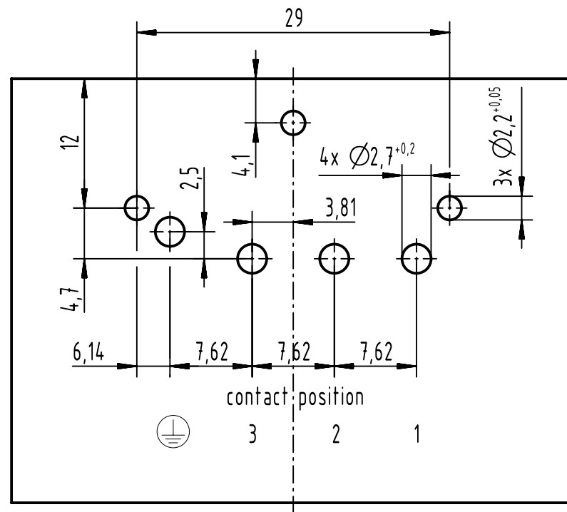
PCB Layout (2:1)
